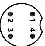
Nor4555 outside view MicroCom connector
