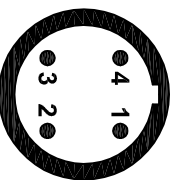
Nor4555 outside view Lemo 00 4 pin connector
